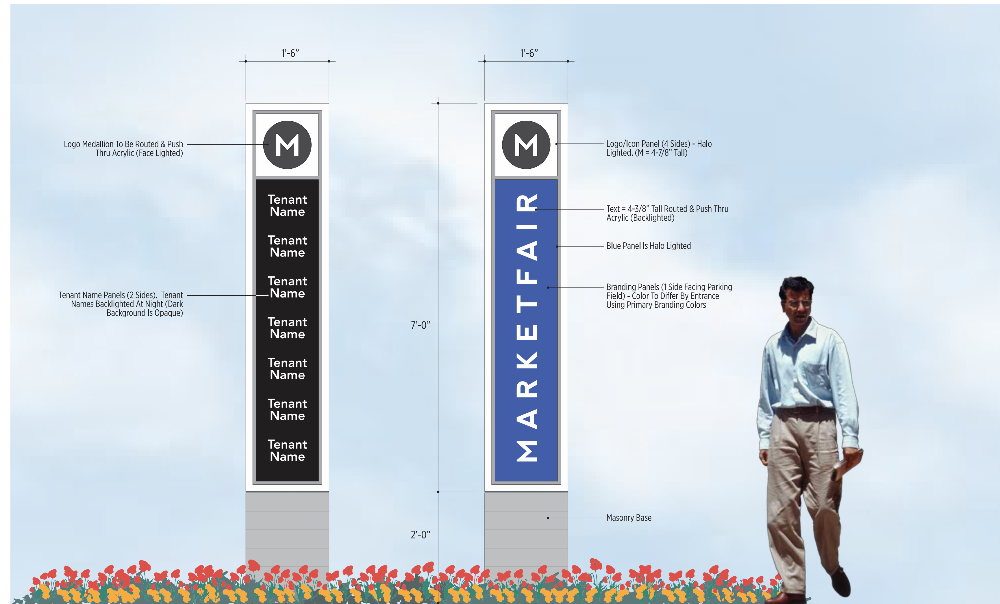
18 19 20 4-Sided Mall Entry Markers @ Recessed Mall Entrances (Internally Illuminated) Scale: 1" = 1'-0"
